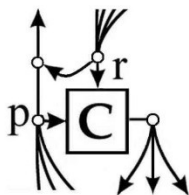
Figure 3. Detail showing branch of reference signal merging with perceptual input.
